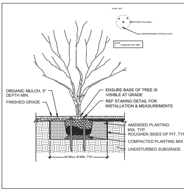
2 | MULTI-TRUNK TREE
