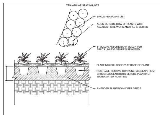
3 | SHRUB PLANTING
