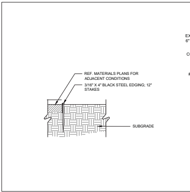
4 | STEEL EDGING
