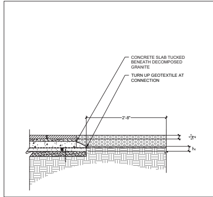
3 | DG TO STONE PAVER TRANSITION 1" = 1'-0" SECTION
