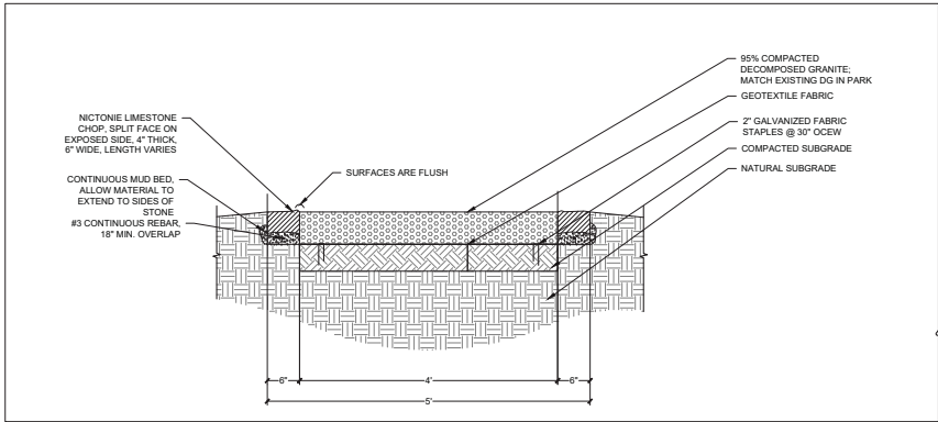
1 | 5' DG PATH WITH STONE CURB 1" = 1'-0" SECTION
