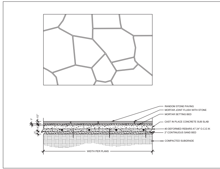
2 | STONE PAVING ON SLAB 1" = 1'-0" SECTION
