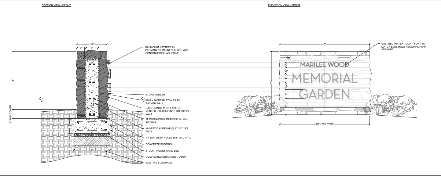
4 | ENTRY SIGN 3/4" = 1'-0" SECTION
