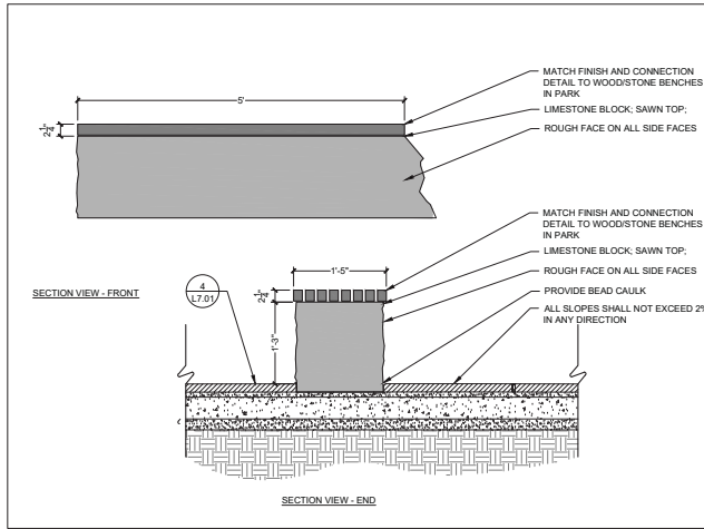
5 | LIMESTONE SEATWALL WITH WOOD TOP
