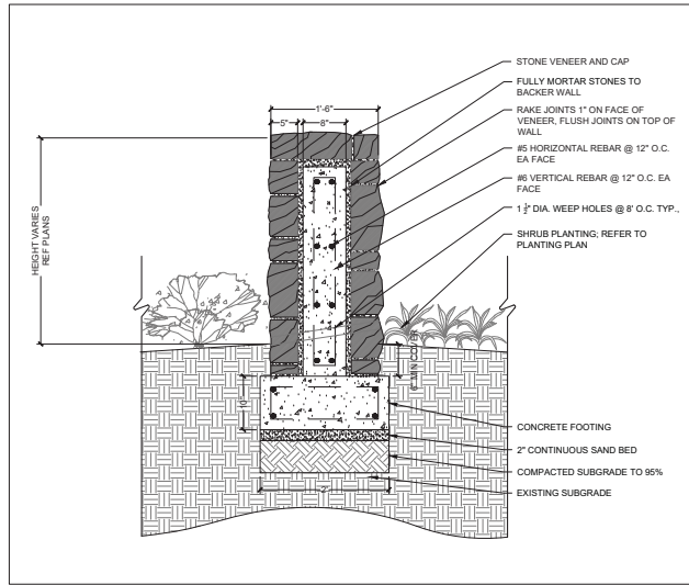
2 | THEMATIC WALL AT SHRUB PLANTING 3/4" = 1'-0" SECTION
